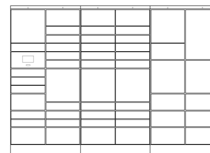
SB214-21 base SB214-22 add-on SB214-11 add-on
